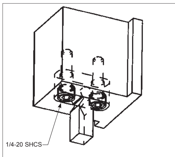
Blind Pocket Retainer used with a custom Lifter
