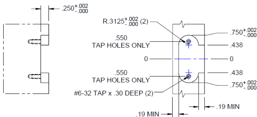
MACHINING FOR LATCH ASSEMBLY INSTALLATION
