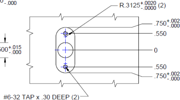
MACHINING FOR HOUSING INSTALLATION
