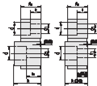
(Normal bushing)
