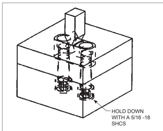
Blind Pocket Retainer in the Ejector Plates
